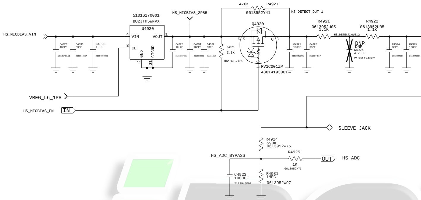
SENSOR HUB HEADSET DETECTION CIRCUIT
